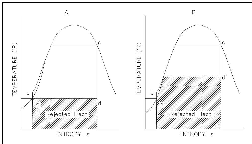
Figure 33 Rankine Cycle Efficiencies T-s
