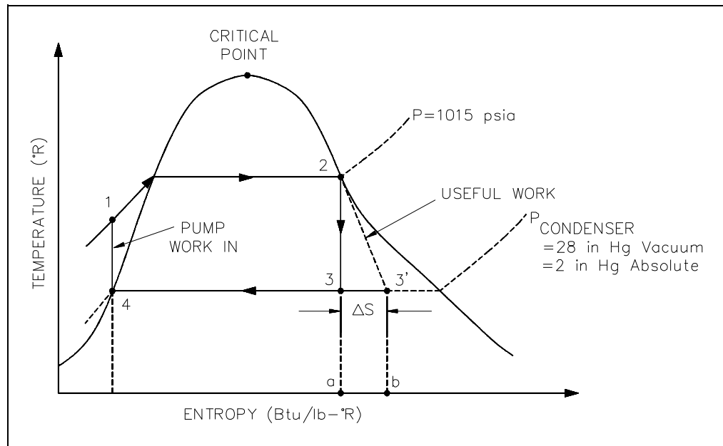
Figure 32 Rankine Cycle With Real v.s. Ideal
